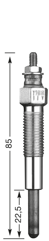
Y-701 R M 10 x 1.25 12 Hex 11 V
