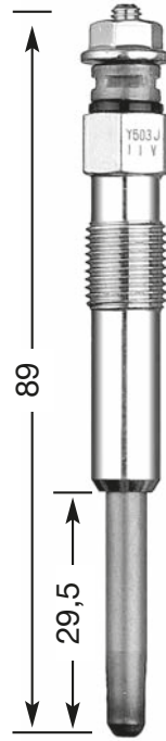
Y-503 J M 10 x 1.0 10 Hex 11 V DP 10
