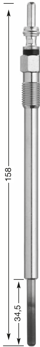
Y-9003 AS M 9 x 1.0 9 Hex 4,4 V DP 78
