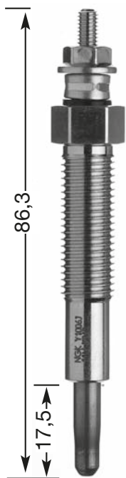
Y1006 J M 10 x 1.25 12 Hex 11 V
