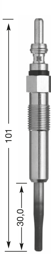
Y-607 AS M 10 x 1.0 10 Hex 5 V DP 50
