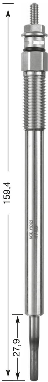
Y1012 J M 10 x 1.25 10 Hex 11 V DP 65
