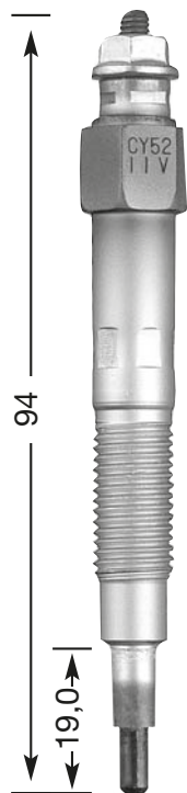
CY 52 M 10 x 1.25 12 Hex 11 V
