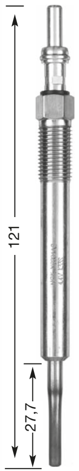
Y9004 AS M 9 x 1.0 9 Hex 4,4 V
