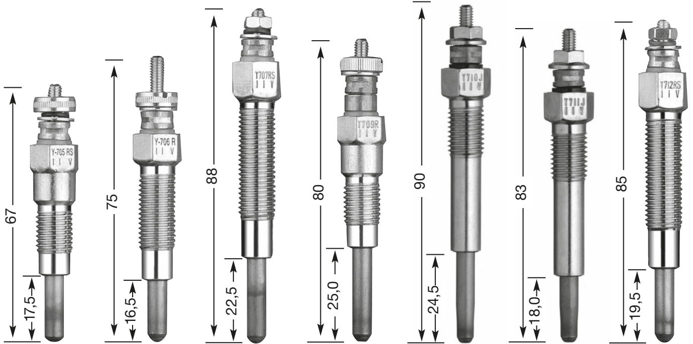
Y-705 RS M 10 x 1.25 12 Hex 11 V
