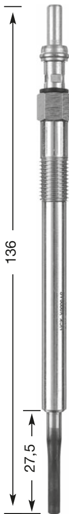
Y8008 AS M 8 x 1.0 8 Hex 11 V DP 74
