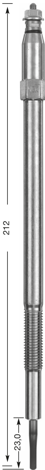
Y-522 J M 10 x 1.25 12 Hex 11 V
