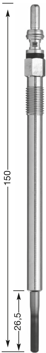
Y8002 AS M 8 x 1.0 8 Hex 4,4 V DP 51
