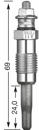
Y-913 J M 12 x 1.25 12 Hex 11 V DP 15
