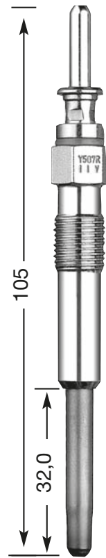
Y-507 R M 10 x 1.0 10 Hex 11 V
