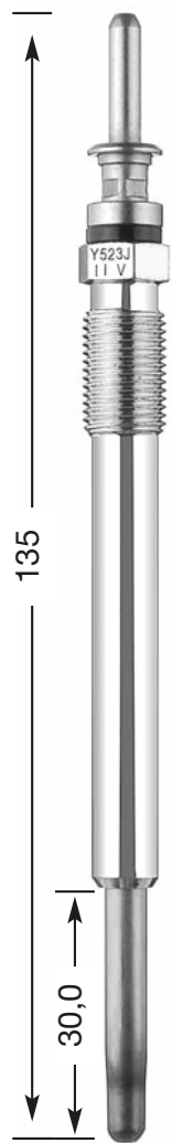
Y-523 J M 10 x 1.0 10 Hex 11 V DP 37
