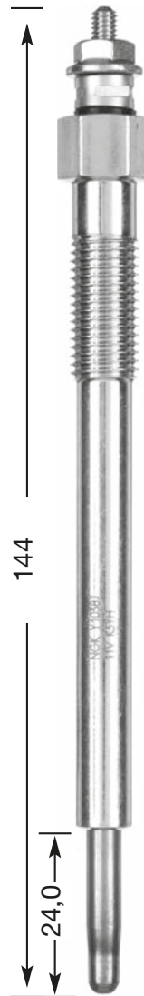
Y1038 J M 10 x 1.25 12 Hex 11 V
