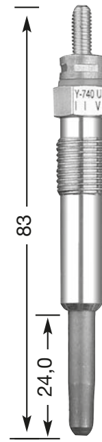
Y-740 U M 10 x 1.0 10 Hex 11 V DP 22
