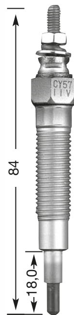
CY 57 M 10 x 1.25 12 Hex 11 V
