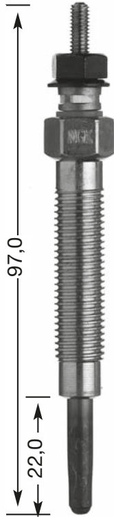
Y-722 JS M 12 x 1.25 12 Hex 11 V
