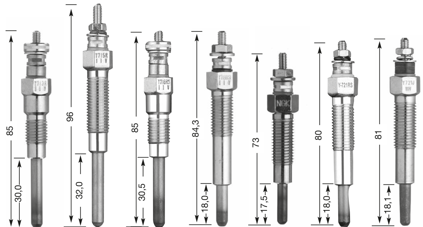
Y-713 R M 10 x 1.25 12 Hex 11 V
