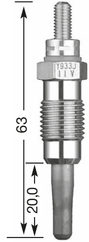
Y-933 J M 12 x 1.25 12 Hex 11 V DP 25
