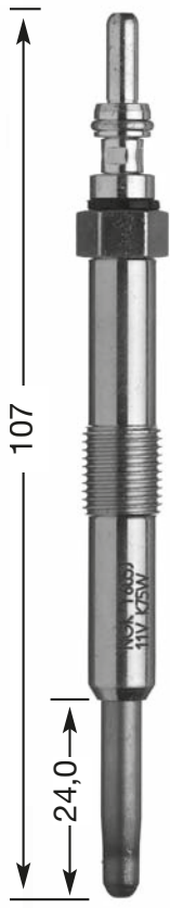
Y-605 J M 10 x 1.0 10 Hex 11 V
