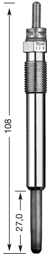
Y-504 R M 10 x 1.0 10 Hex 11 V DP 24
