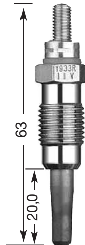
Y-933 R M 12 x 1.25 12 Hex 11 V DP 25
