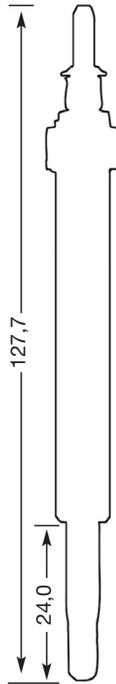
Y-609 AS M 10 x 1.0 7,5 V DP 49
