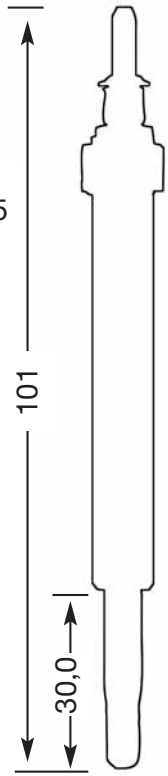
Y-607 AS M 10 x 1.0 10 V
