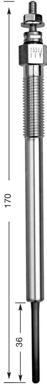
Y-531 J M 10 x 1.25 12 Hex 11 V
