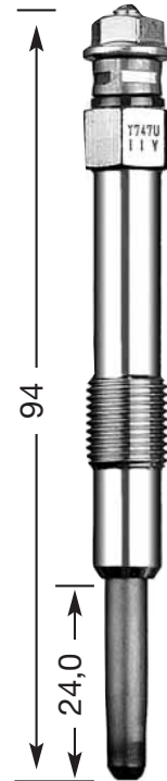
Y-747 U M 10 x 1.0 10 Hex 11 V DP 26
