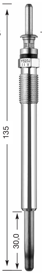
Y-523 J M 10 x 1.25 10 Hex 11 V DP 37
